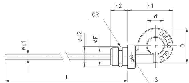
Version 480082 - 1 O-ring.
