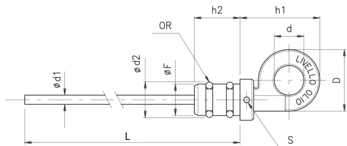
Version 480084 - 2 O-rings.
