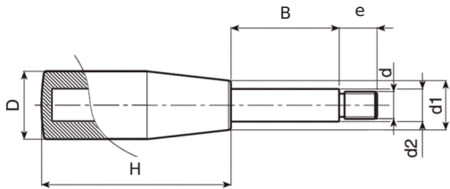
PA Black reinforced polyamide. Threaded zinc plated steel stud.
