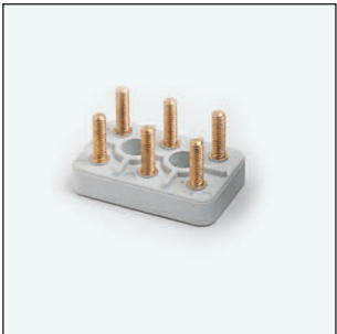
Synthetic material F531 DIN 7708. Brass studs. Terminal links for this block 110094 / 390019.
