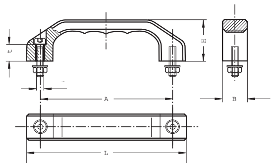
VERSION AG-F FRONT MOUNTING
